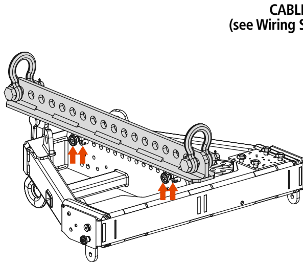
FRONT POSITION
