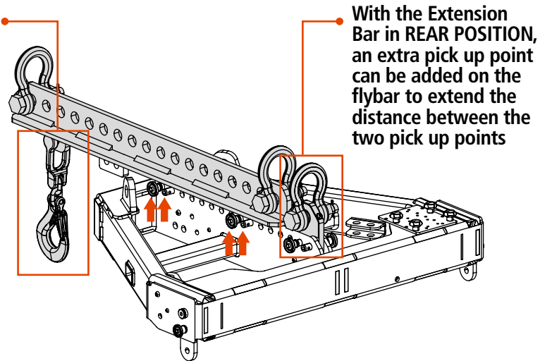
REAR POSITION
